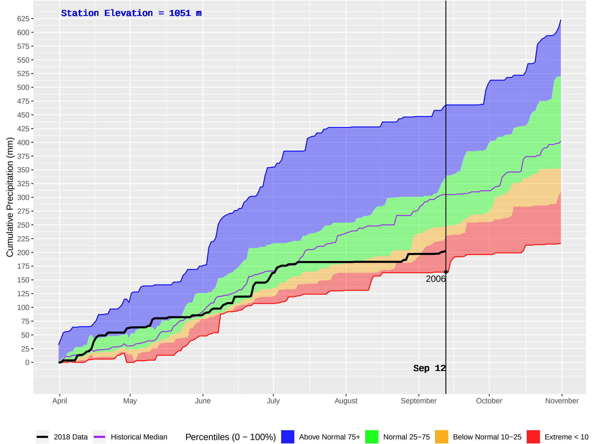
GOATHAVEN (886) : Historical (2005–2016) and Current (2018) Daily Cumulative Precipitation
